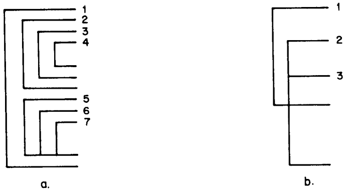
Figure 13 DO Loops
