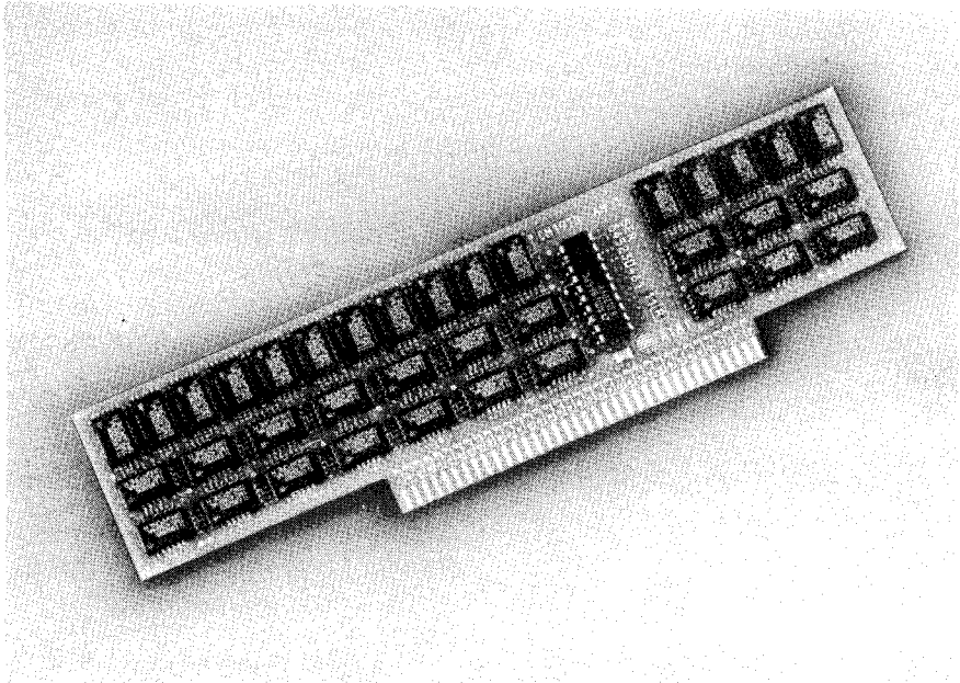
Figure 3-5. Back Side of a 2-Megabyte RAM Card
